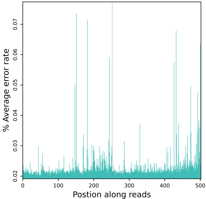
Error rate distribution along reads (R20220)
